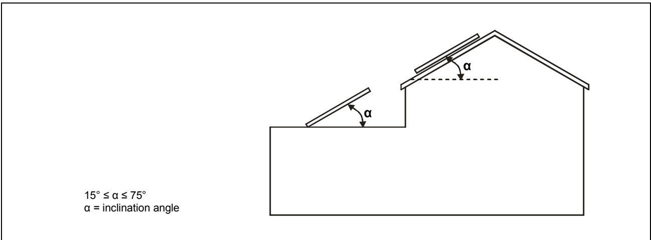
fig. 20 – Inclination of collectors
