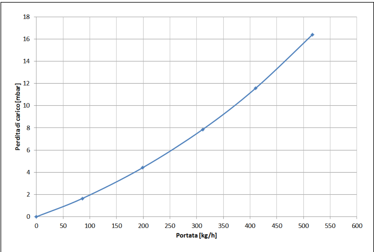
fig. 19 - Pressure losses
