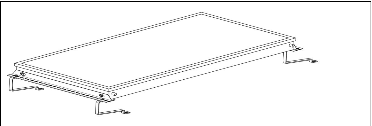
fig. 25 - Roof installation without wood-blocks
