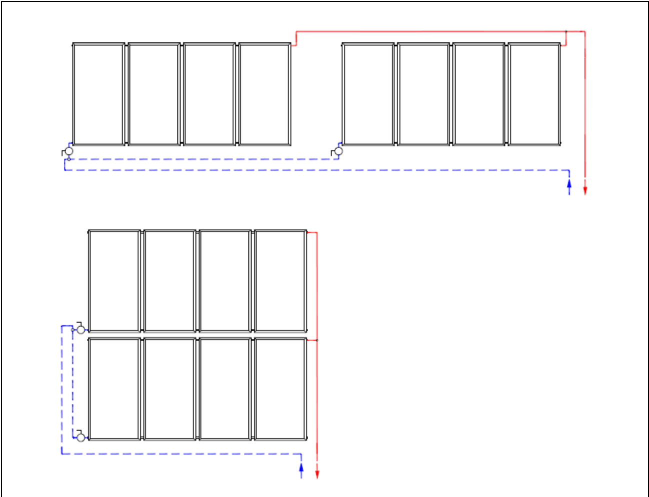
fig. 23 - Examples of collector fields connected in series/parallel
