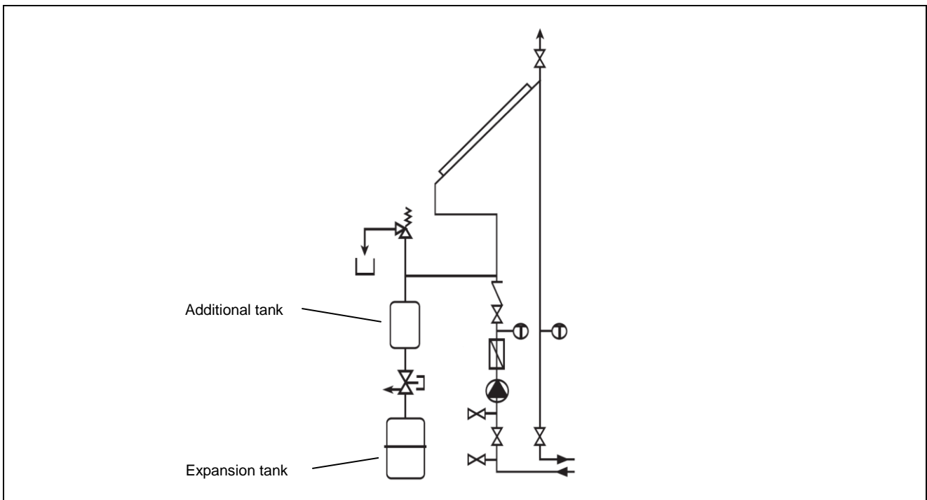
fig. 32 - Expansion tank
