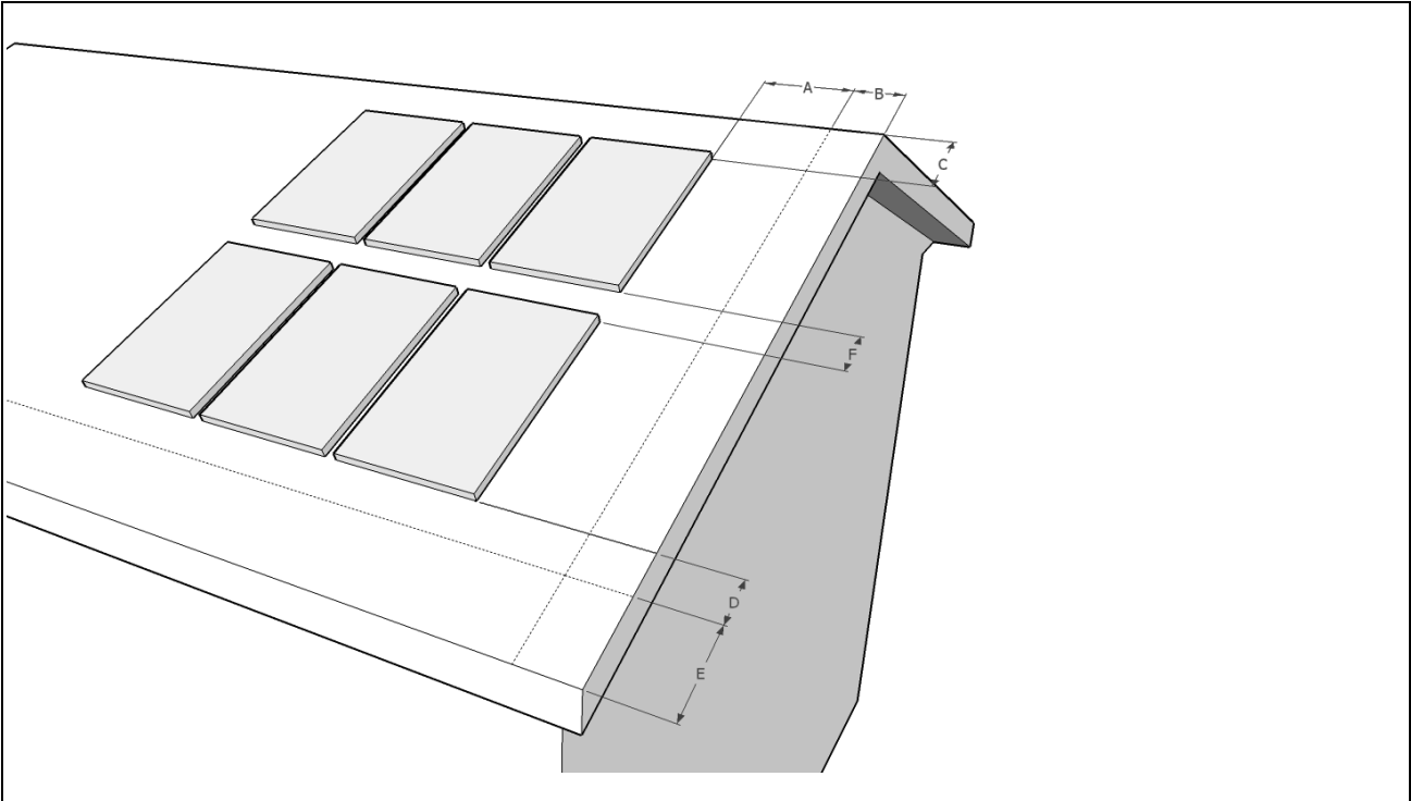
fig. 21 - Installation distances
