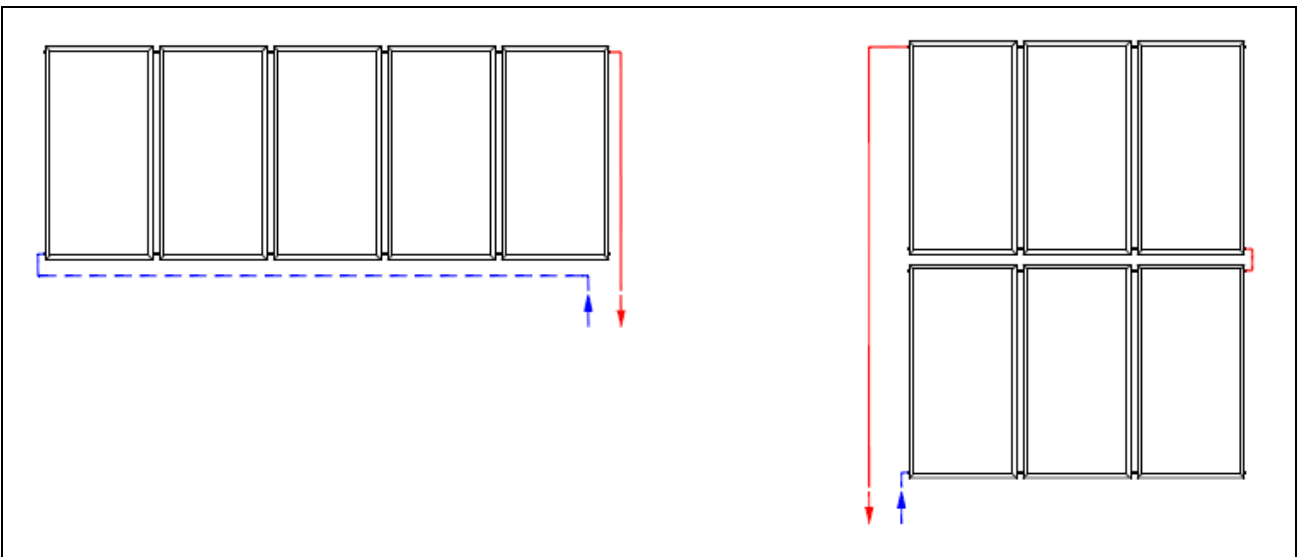
fig. 22 - Examples of collector fields
